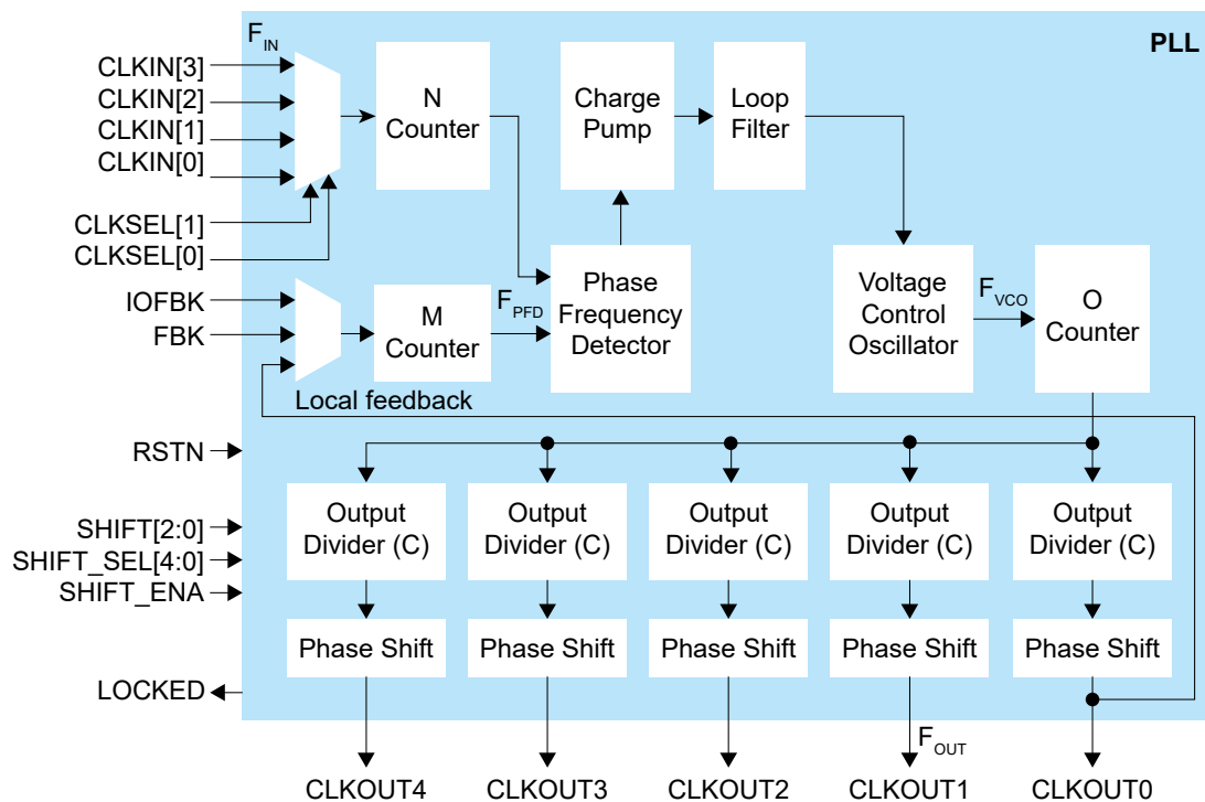
Figure 24: PLL Block Diagram
