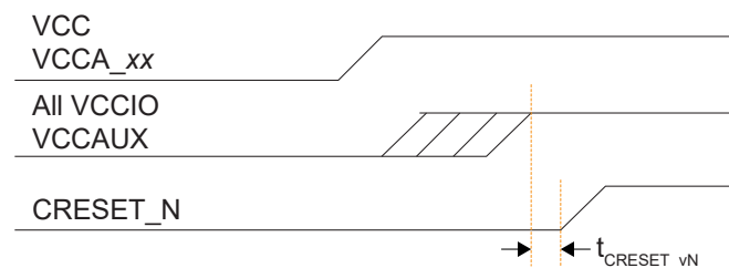
Figure 31: Power Up Sequence
